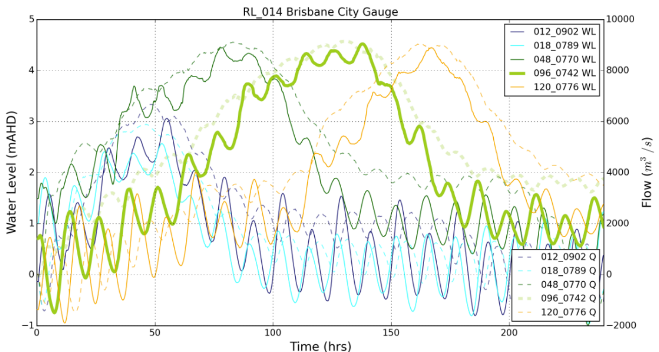
Figure 7-4 Hydrograph (Stage and Flow) at Brisbane City Gauge for the 1 in 100 AEP Ensemble (5 Events)
